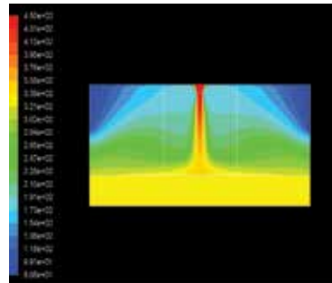
Standard Air Impingement Oven
